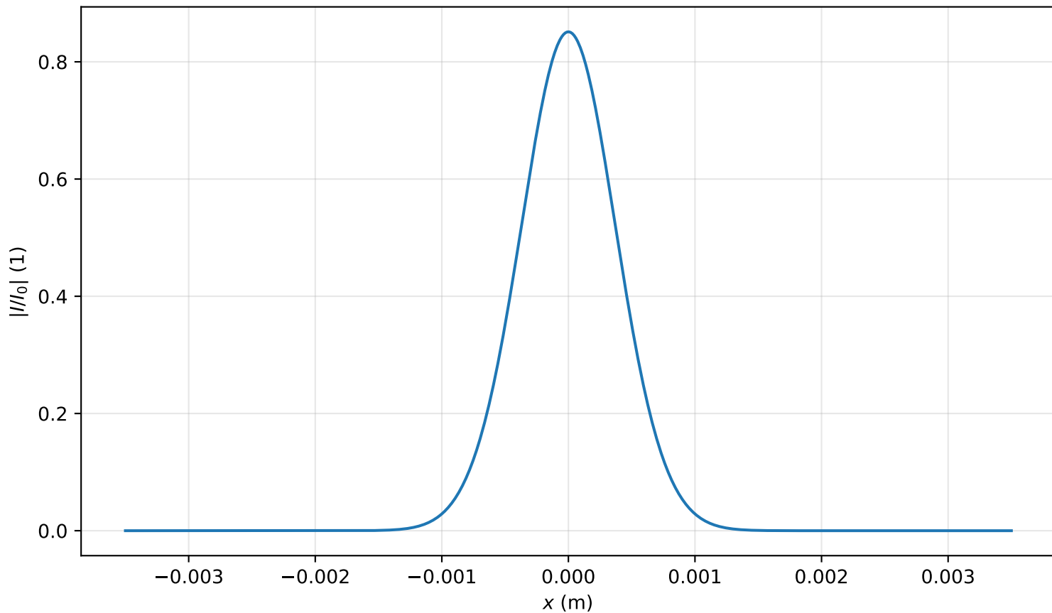
Intensity profile I(x, y = 0, z = 0.955m)/I_0 , P_{in}=0.1P_{cr} , artificial time
